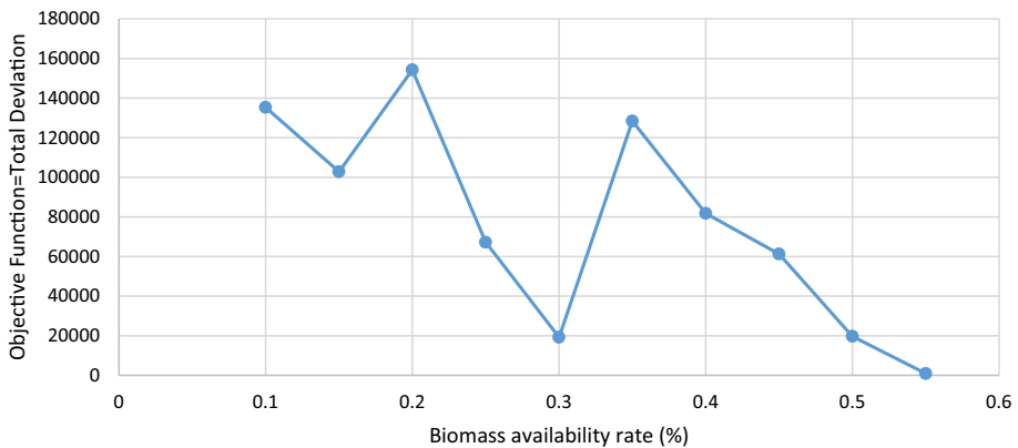
Fig. 7 The effect of biomass amount on the number of facilities and objective function value
