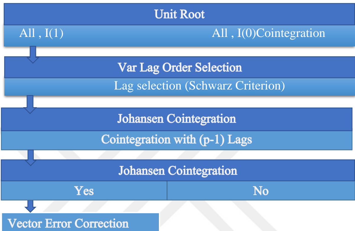
Figure 3.1. Steps for Empirical Analysis
