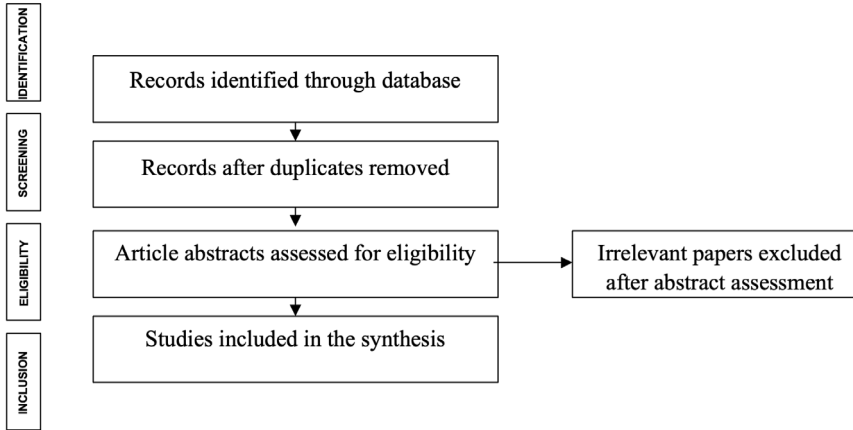
Figure 1: PRISMA Flowchart.
