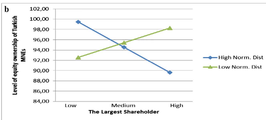
Fig. 2b. The interaction between CONCEN and NRMDIST.
