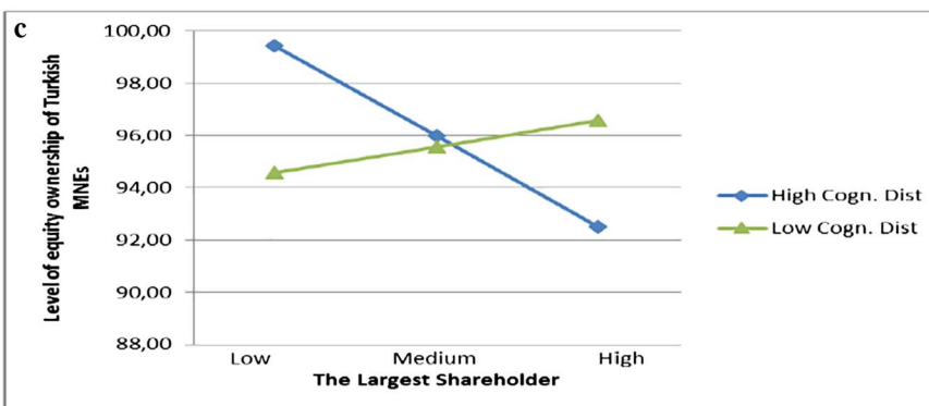
Fig. 2c. The interaction between CONCEN and COGDIST.
